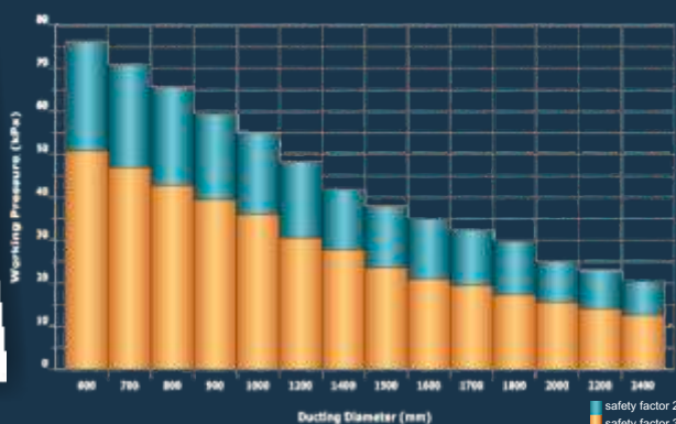
MAT HELLAS Ventilation Ducting Pressure Chart Highest permitted working pressure
